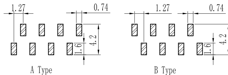
PCB LAYOUT
