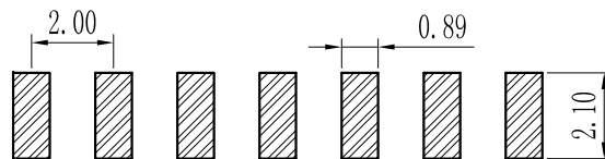
PCB LAYOUT
