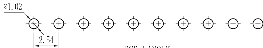
PCB LAYOUT
